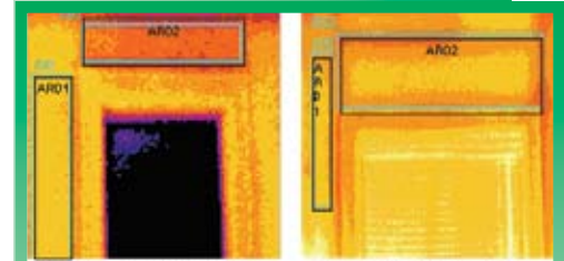
Wood-Framed Home The temperature difference between the insulation (AR01) and the window header (AR02) is 1.9°C
